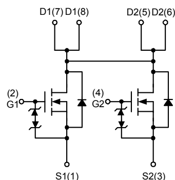
N-Channel MOSFET
