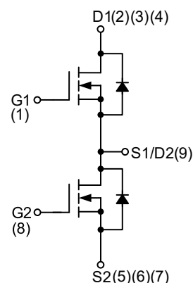
N-Channel MOSFET
