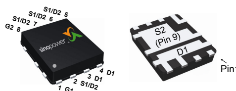
DFN5x6E-8_EP2
