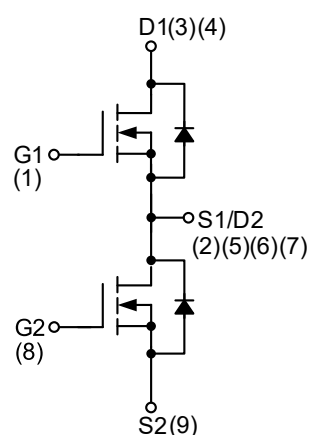
N-Channel MOSFET
