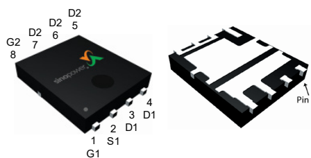
DFN5x6J-8_EP2
