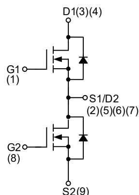
N-Channel MOSFET
