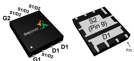
DFN5x6G-8_EP2
