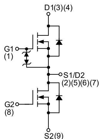
N-Channel MOSFET
