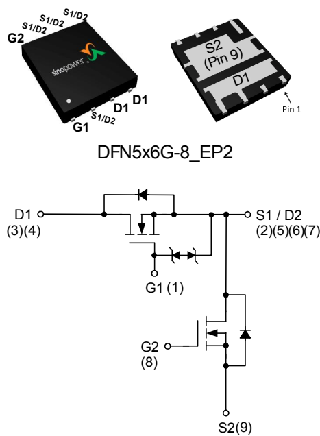
N-Channel MOSFET
