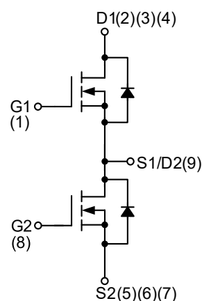
N-Channel MOSFET
