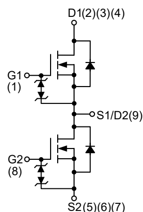
N-Channel MOSFET
