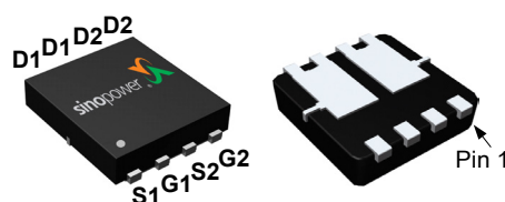
DFN5x6C-8_EP2
