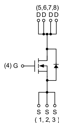
N-Channel MOSFET
