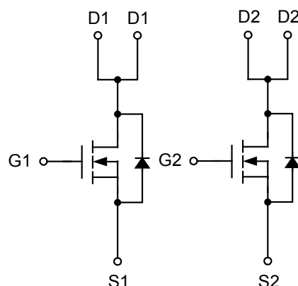
N-Channel MOSFET
