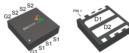
DFN3x3H-8_EP2
