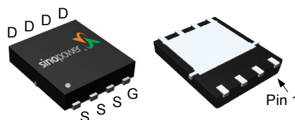
DFN5x6A-8_EP
