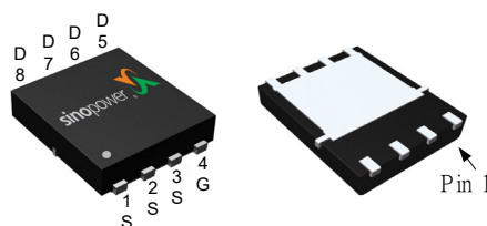
DFN5x6A-8_EP
