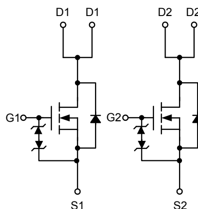
N-Channel MOSFET
