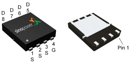
DFN5x6A-8_EP
