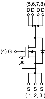
N-Channel MOSFET
