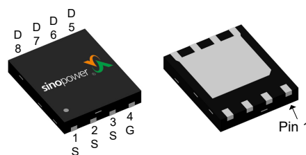
DFN5x6O-8_EP
