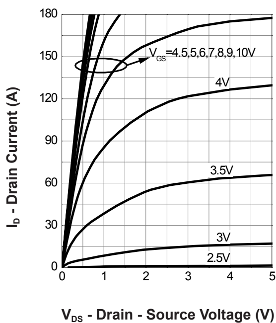
Output Characteristics
