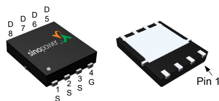
DFN5x6A-8_EP
