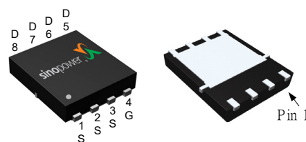
DFN5x6A-8_EP
