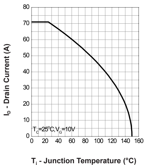
Drain Current
