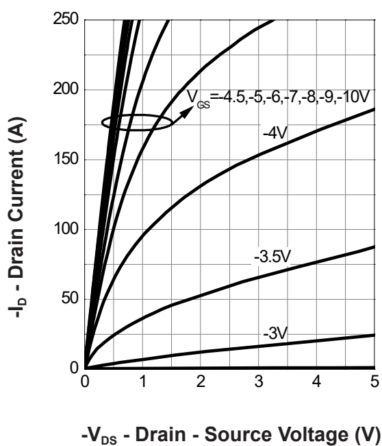
Output Characteristics
