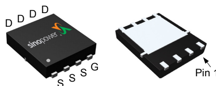
DFN5x6A-8_EP
