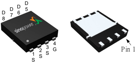
DFN5x6A-8_EP
