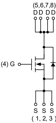
N-Channel MOSFET
