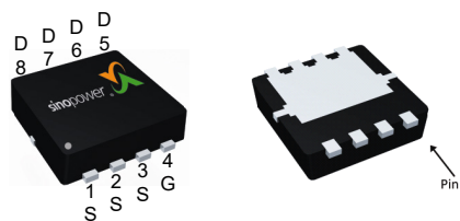
DFN3.3x3.3A-8_EP
