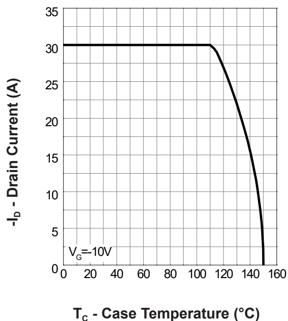
Drain Current
