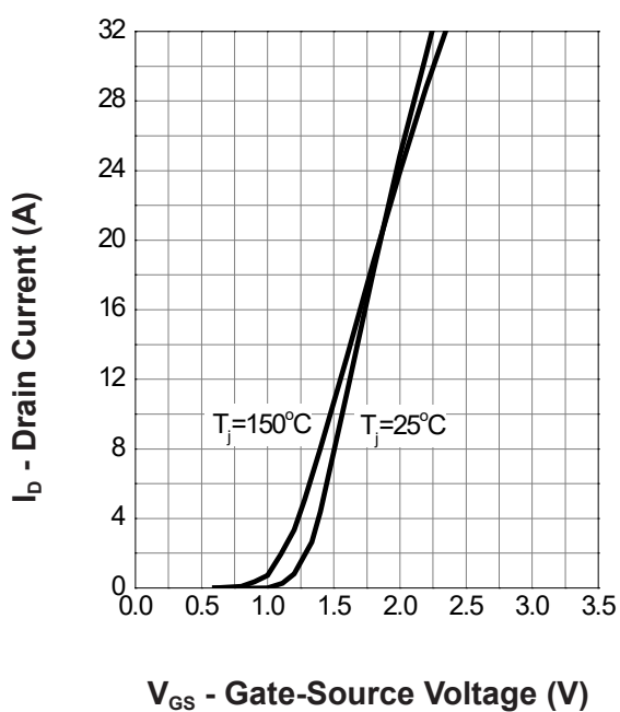
Transfer Characteristics
