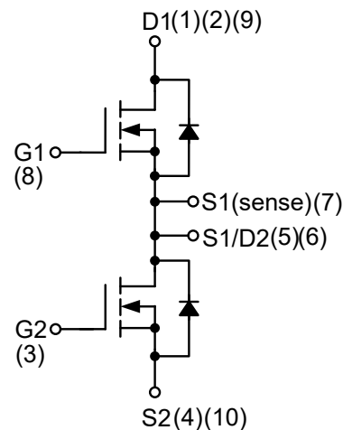
N-Channel MOSFET
