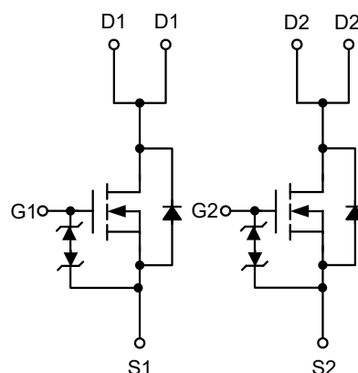
N-Channel MOSFET
