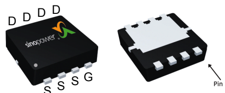
DFN3.3x3.3A-8_EP
