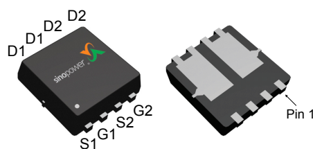
DFN3.3x3.3G-8_EP2
