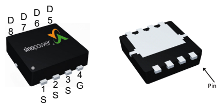
DFN3.3x3.3A-8_EP
