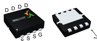
DFN3.3x3.3A-8_EP
