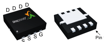
DFN3.3x3.3C-8_EP
