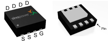
DFN3.3x3.3B-8_EP
