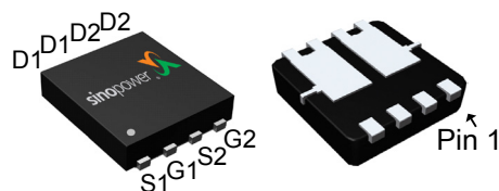
DFN3x3B-8_EP2
