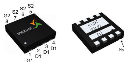
DFN3x3E-8_EP2
