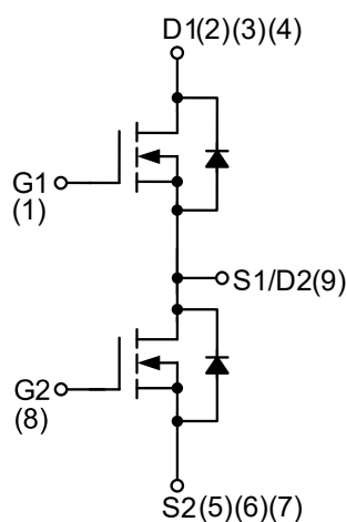
N-Channel MOSFET
