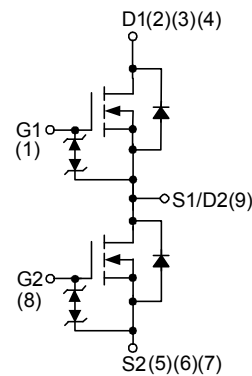
N-Channel MOSFET
