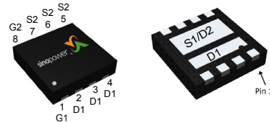
DFN3x3E-8_EP2
