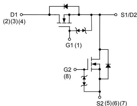
N-Channel MOSFET
