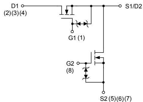
N-Channel MOSFET
