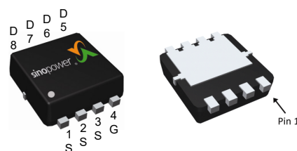
DFN3x3A-8_EP
