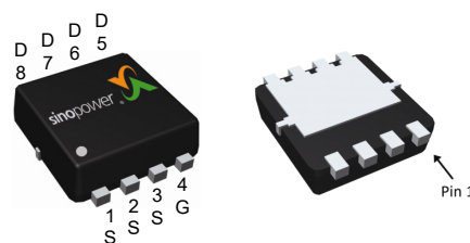
DFN3x3A-8_EP
