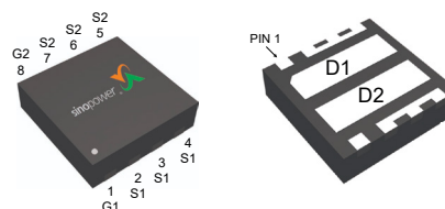
DFN3x3H-8_EP2
