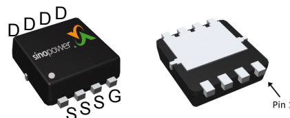
DFN3x3A-8_EP
