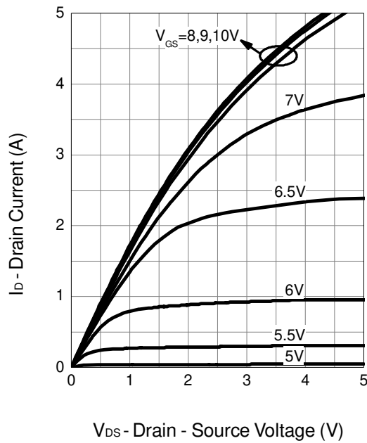
Output Characteristics
