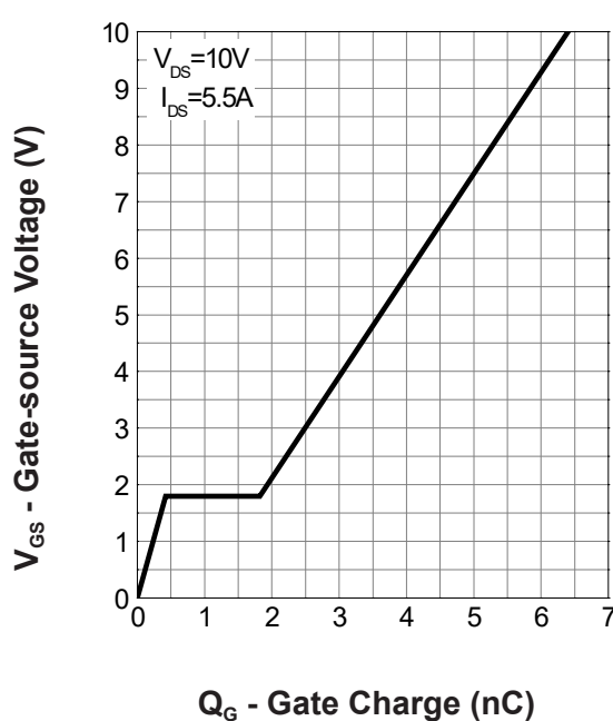
Gate Charge
