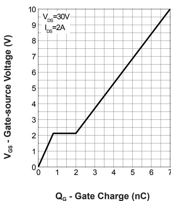
Gate Charge
