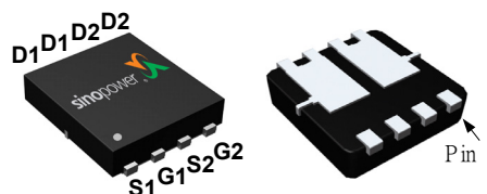
DFN5x6C-8_EP2
