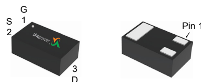
DFN0.6x1-3_EP
